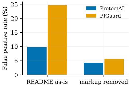
Benign README chunks
