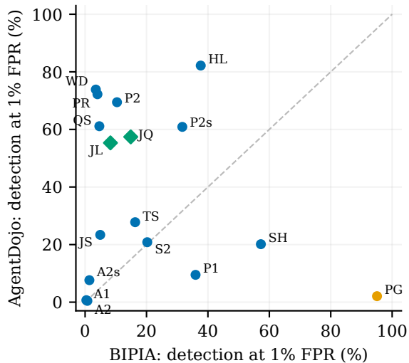
(a) Kendall \tau = 0.01
