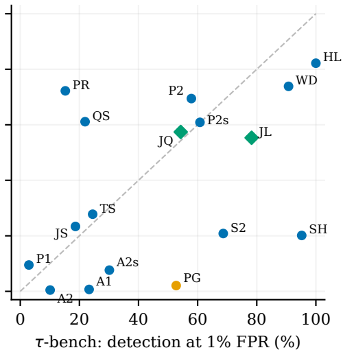
(b) Kendall \tau = 0.28
