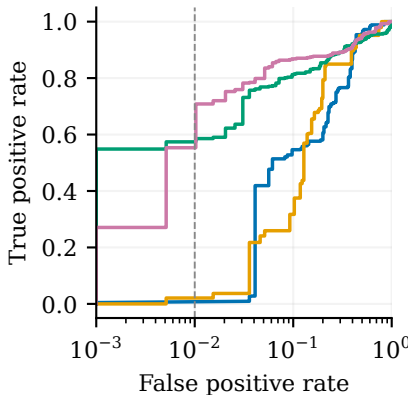
AD-Matched
