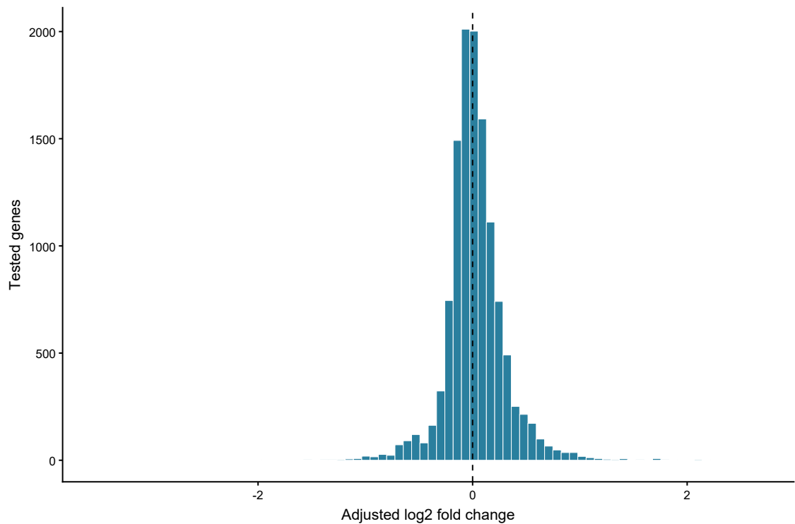
Adjusted gene-effect distribution
