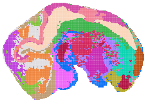
GraphST
