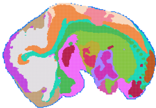
BANKSY
