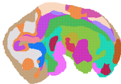
MENDER
