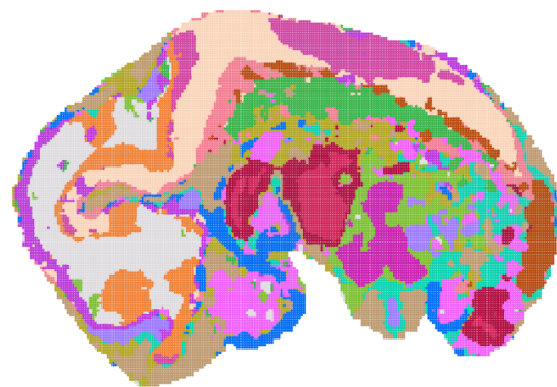
Novae
