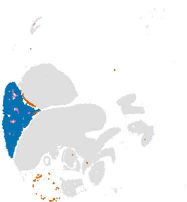
g8 | IoU 0.894
