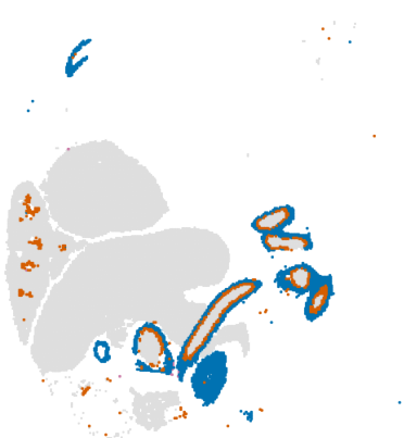
g8 | IoU 0.779
