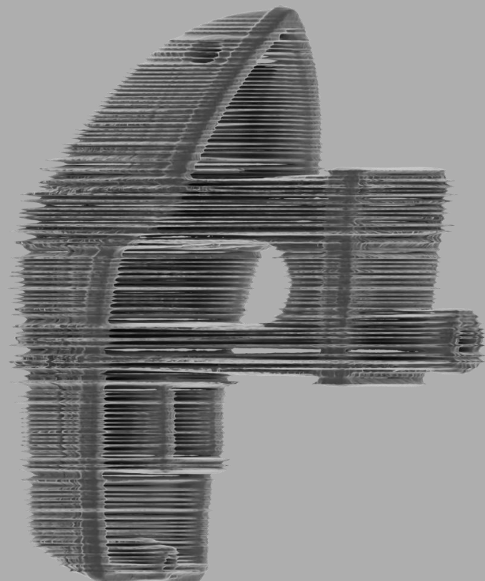
Striations in final part
