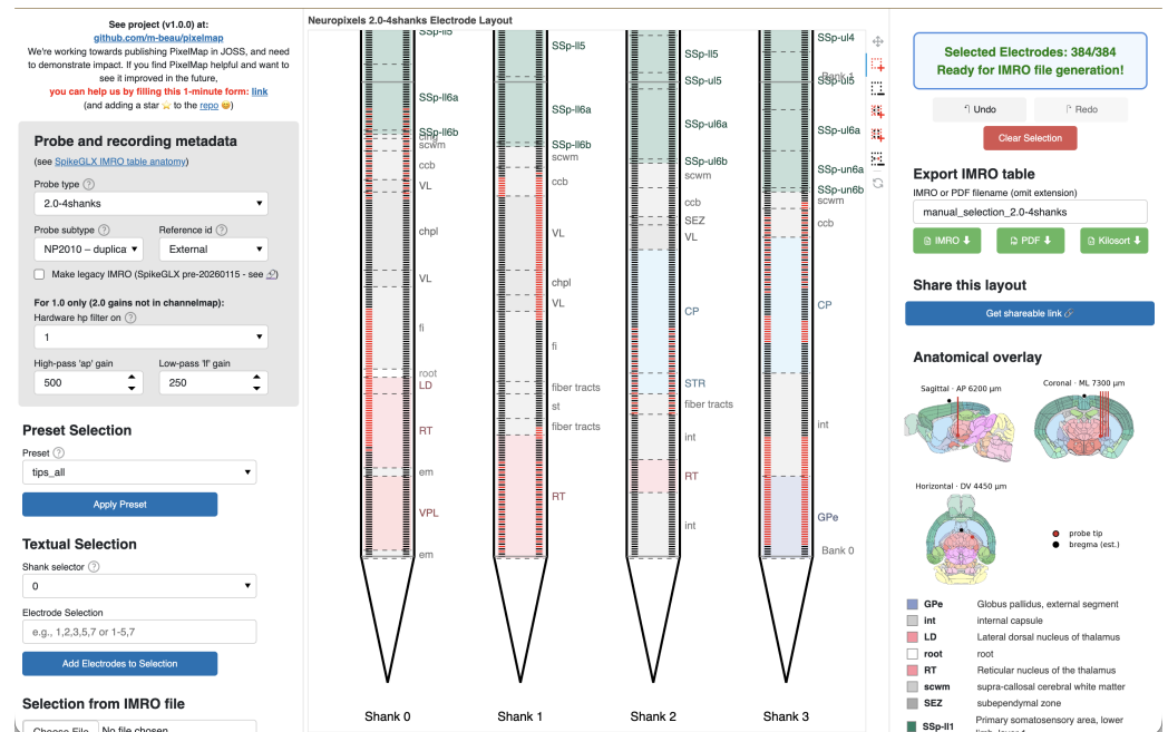
Figure 1: PixelMap's browser-based graphical user interface.
