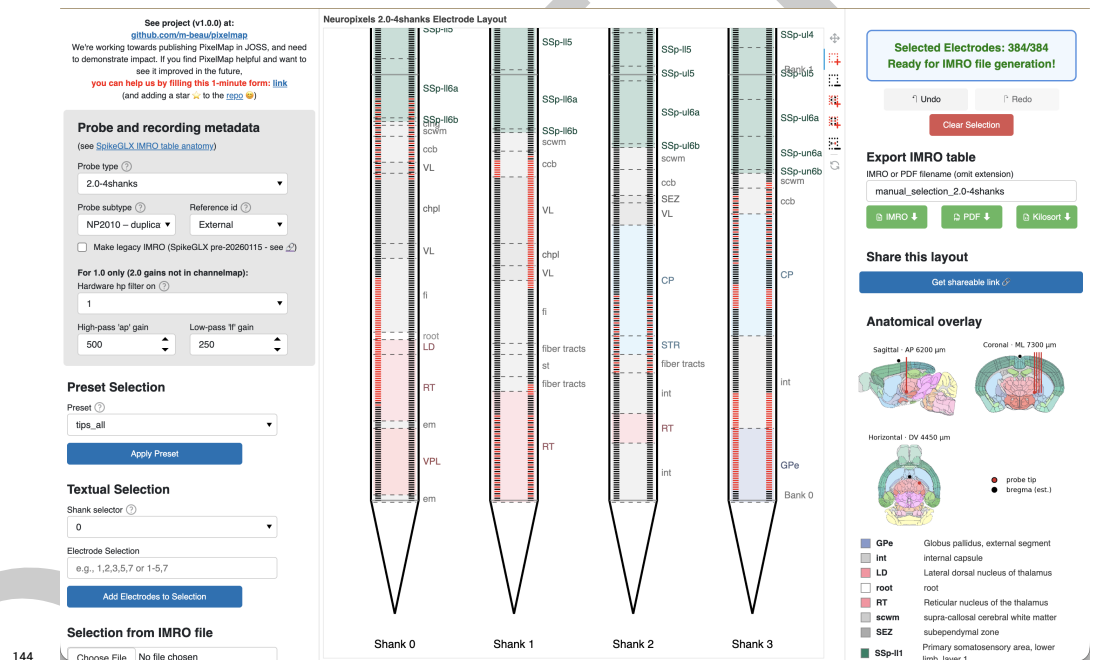
Figure 1: PixelMap's browser-based graphical user interface, shown here for a four-shank Neuropixels 2.0 probe.
