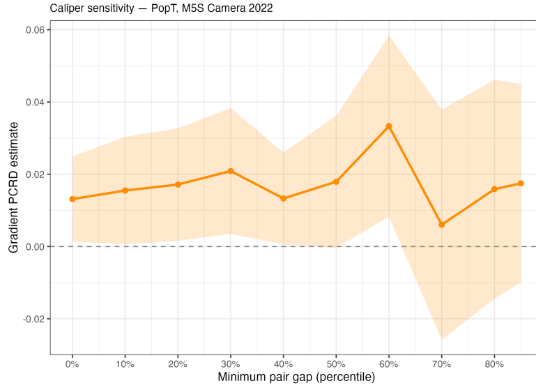
Figure 30: Caliper sensitivity for the gradient PCRD in the overall populism design, outcome: M5S Camera 2022 vote share.
