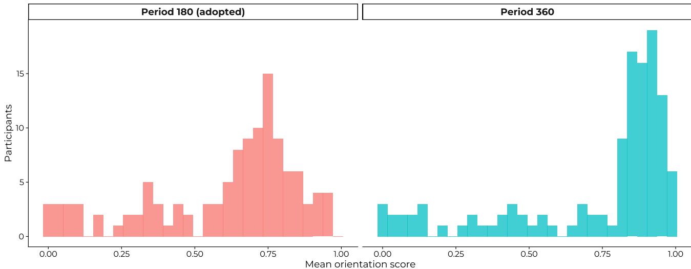
Orientation score under the two angular periods
