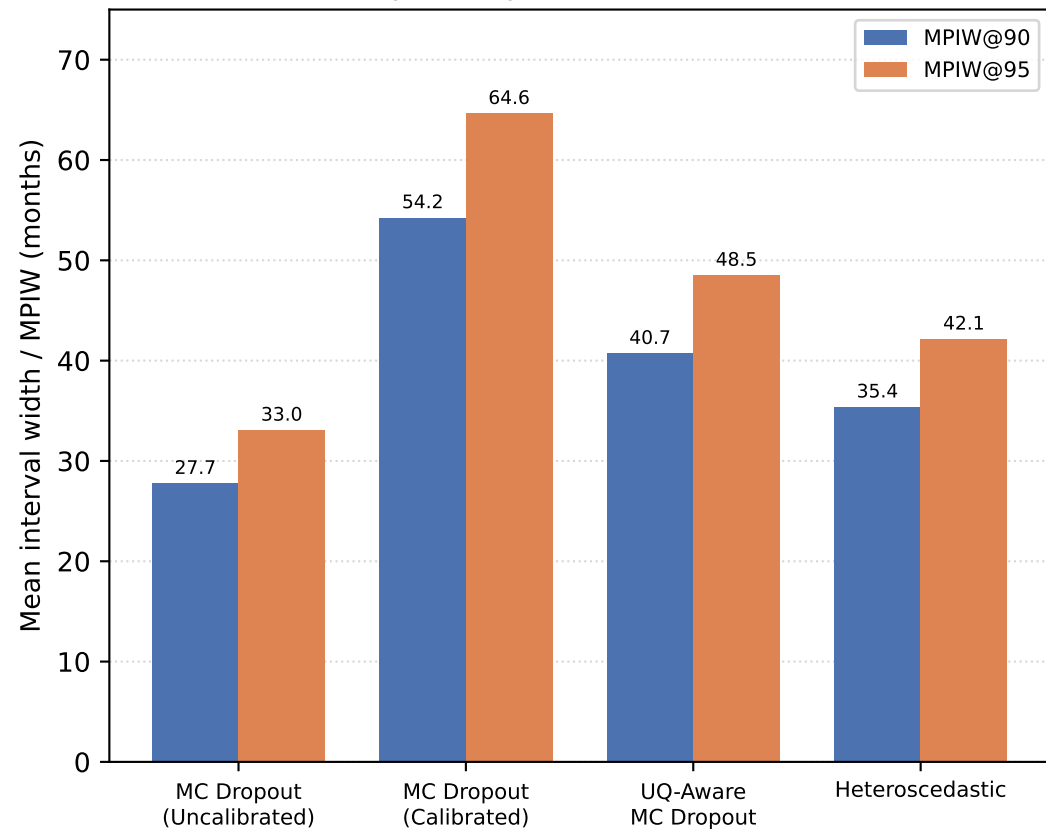
(b) Sharpness: prediction interval width
