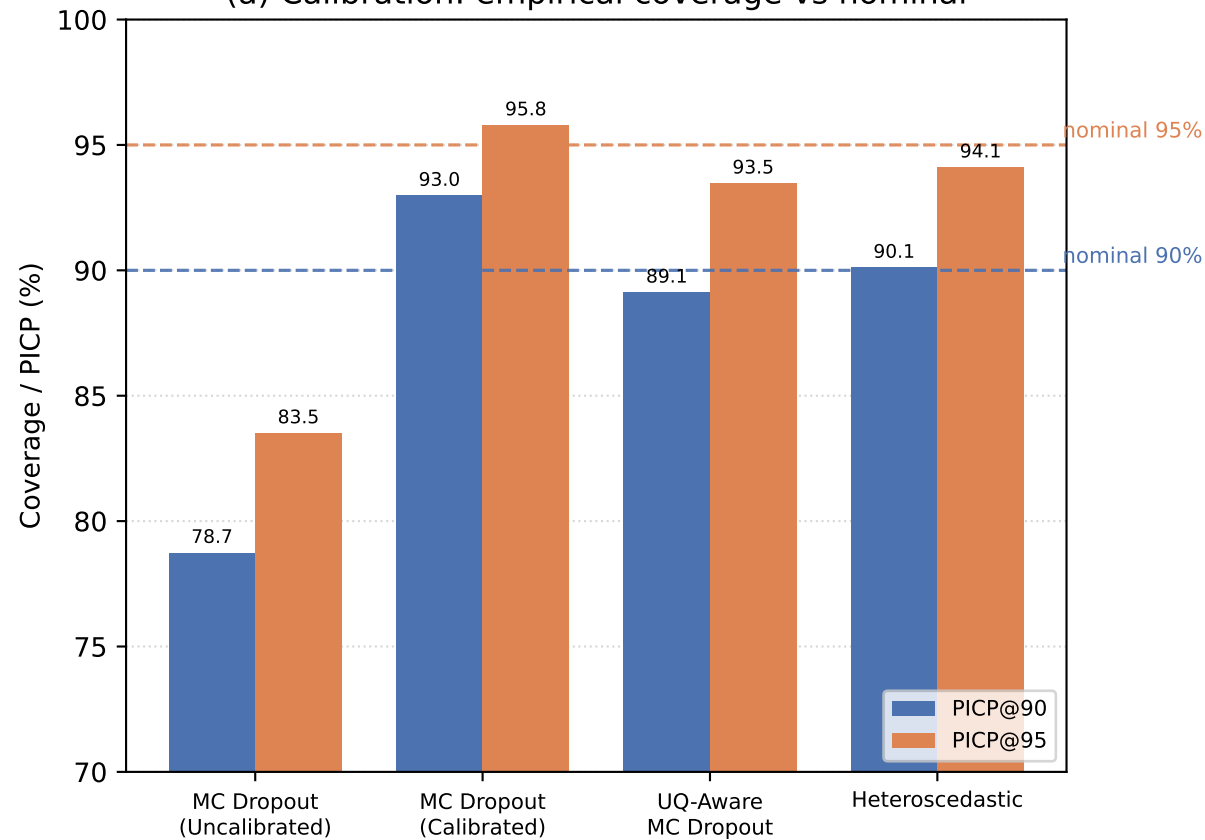
(a) Calibration: empirical coverage vs nominal
