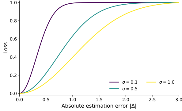
Figure S46: Inverted Gaussian loss functions based on Körding and Wolpert [12], Acerbi et al. [1], for different values of \sigma (Equation 122).
