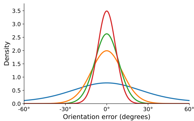
Figure S37: Sensory-noise distributions used in our simulations. In line with our circular simulations, we display them on the orientation scale, i.e., the stimulus space [0^\circ, 180^\circ] . Colors match the model fit plots.
