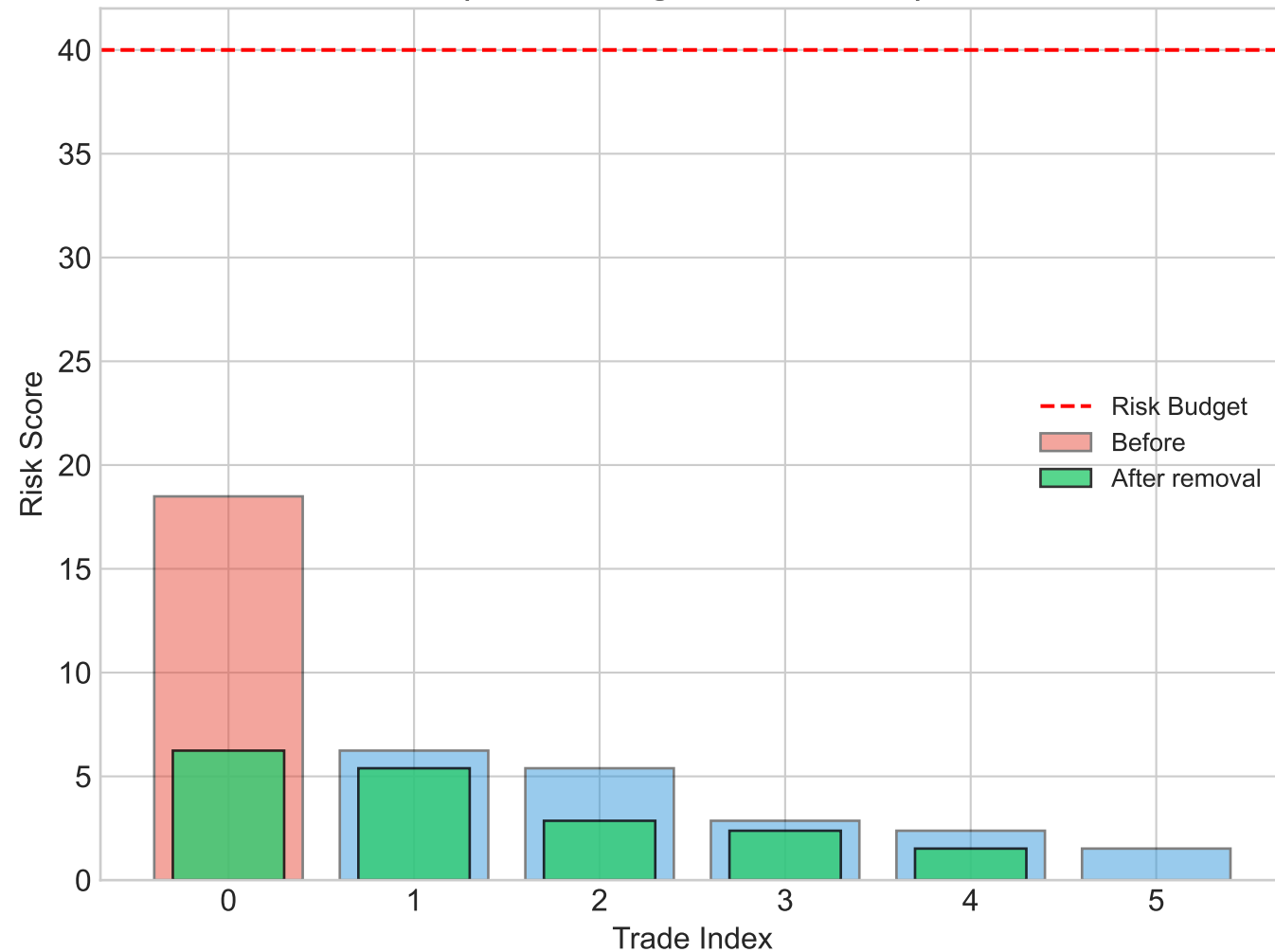
Greedy Risk Enforcement (Remove highest-risk trade)
