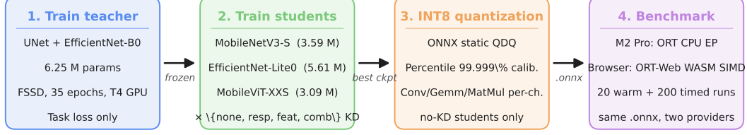
Figure 1: FloodLite training-and-deployment pipeline. Train teacher (UNet+EfficientNet-B0) → train students (three lightweight backbones × four KD configurations) → INT8-quantize the no-KD students via ONNX static QDQ → benchmark FP32 and INT8 on Apple M2 Pro CPU and in browser WebAssembly. Each stage produces an artifact consumed by the next; the same .onnx file is benchmarked under two execution providers (ONNX Runtime CPU on M2 Pro; ONNX Runtime Web WASM SIMD in the browser).
