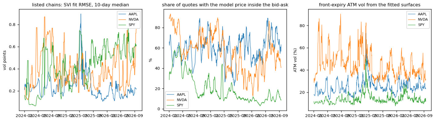
Listed chains (SPY, AAPL, NVDA, daily since 2024): SVI fit RMSE, the share of quotes with the model inside the bid-ask, front ATM vol.
