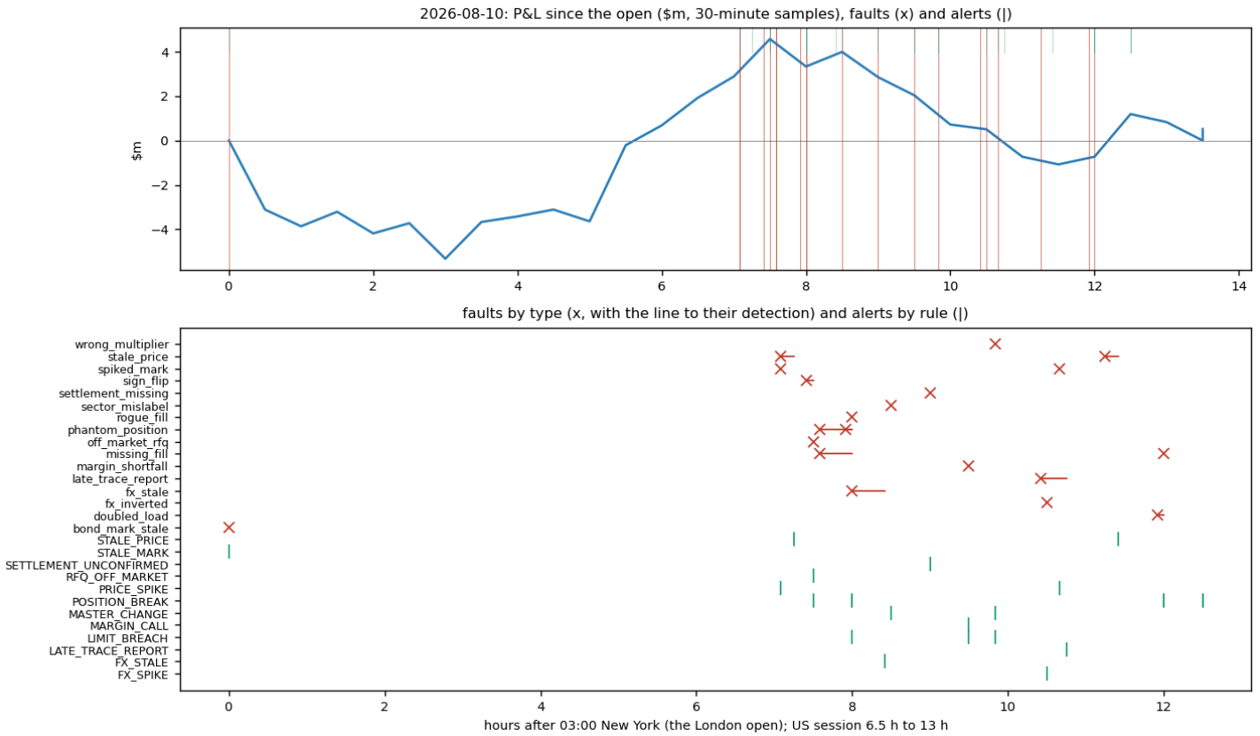
One fault day: P&L since the open with the faults and the alerts, then faults by type with the line to their detection and alerts by rule.
