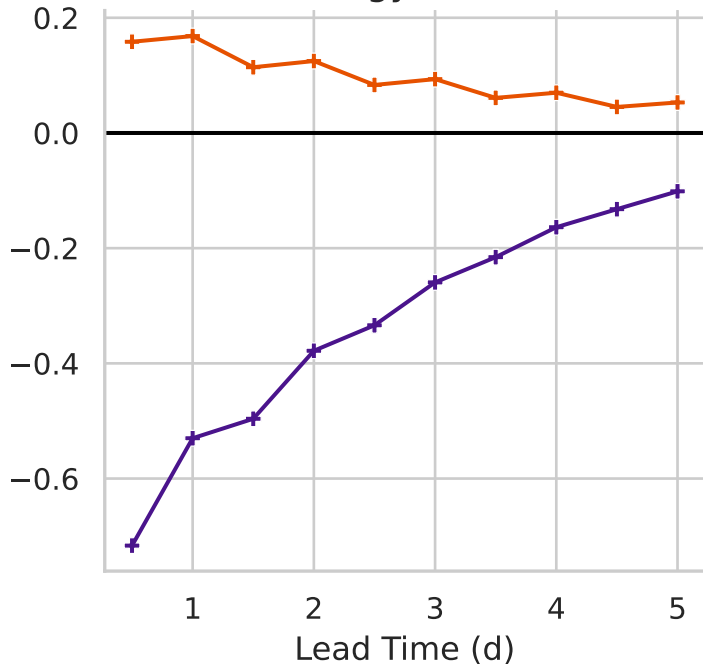
Energy Score
