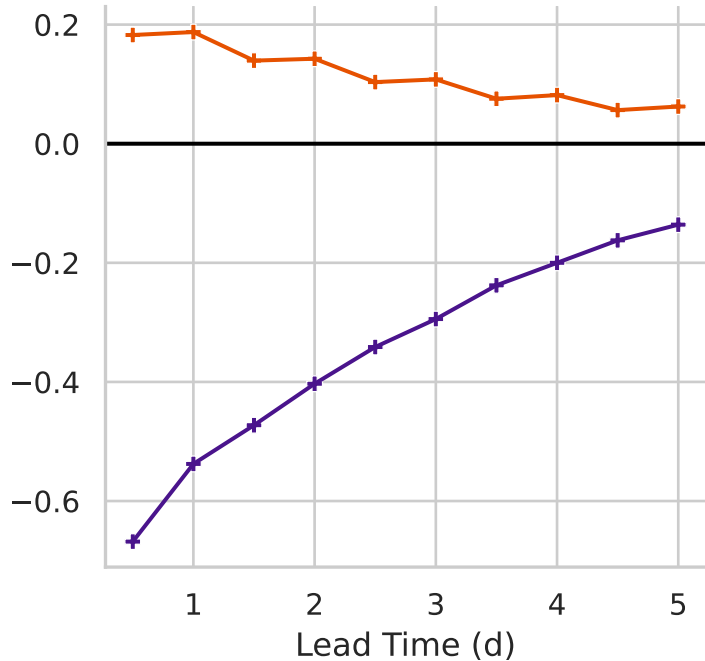
CRPS
