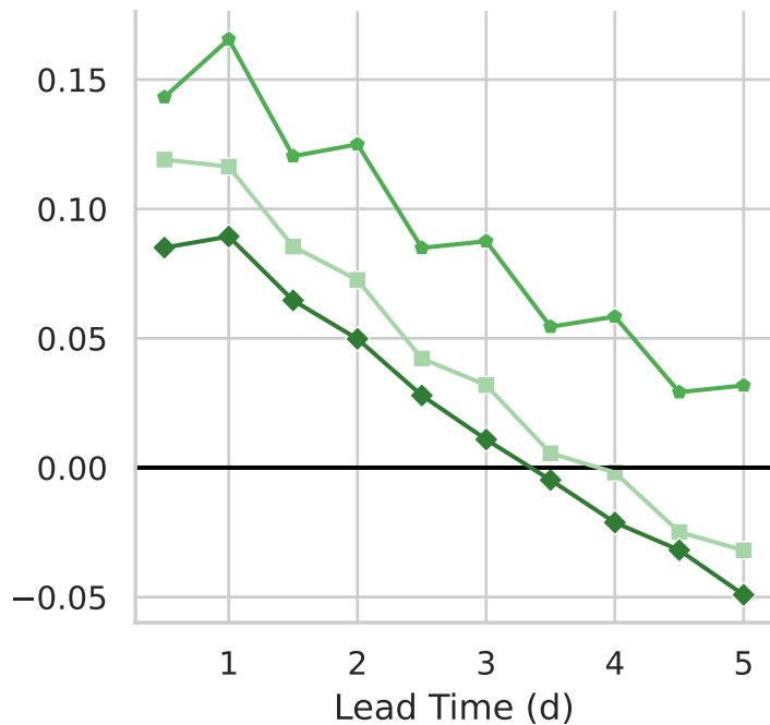
CRPS
