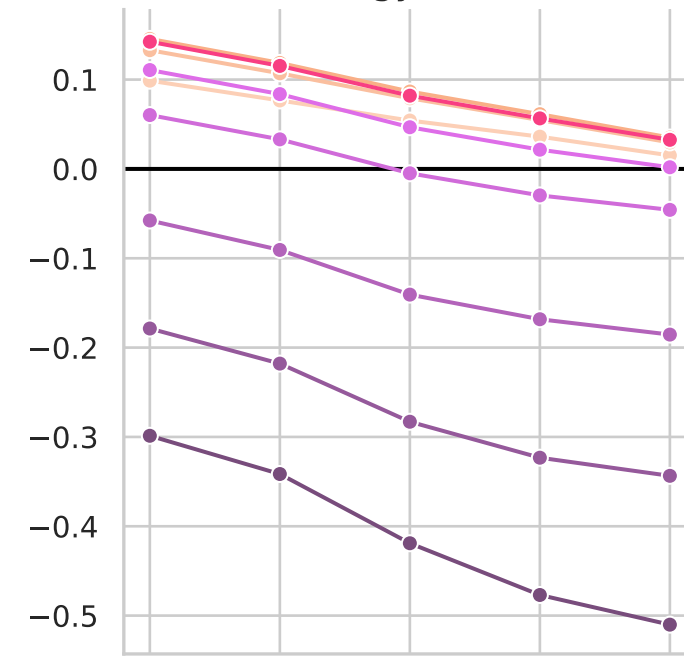
Energy Score
