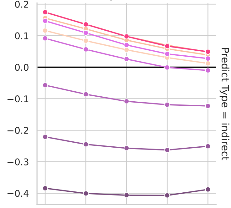
Variogram Score
