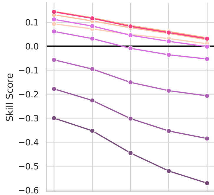
CRPS
