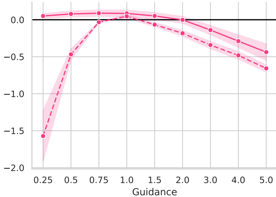
CRPS
