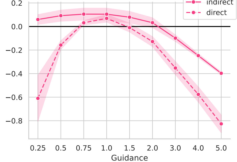
Variogram Score
