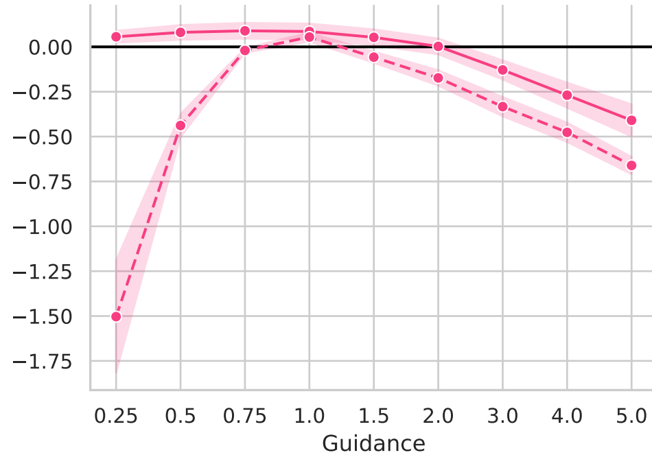
Energy Score
