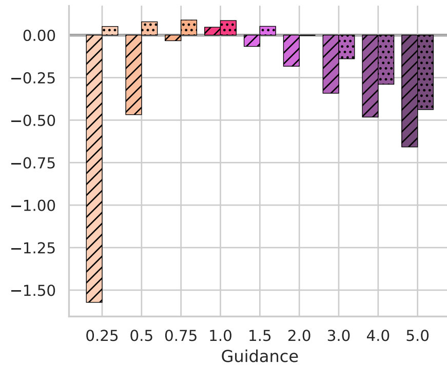
CRPS
