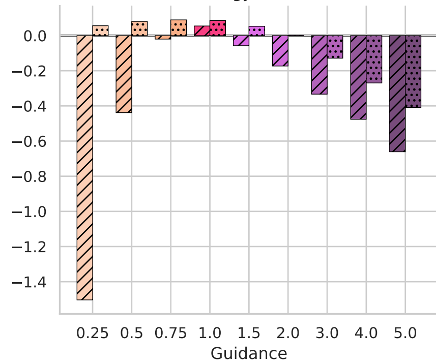
Energy Score
