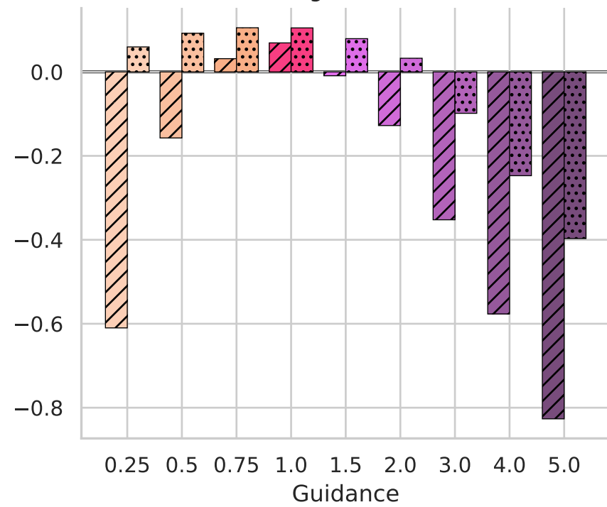
Variogram Score
