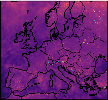
ENGRESSION (IND)
