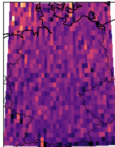
ENGRESSION (ES)
