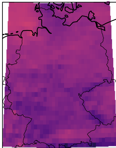
DRN
