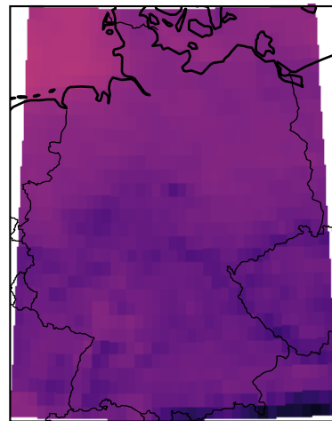
FM (UNET)
