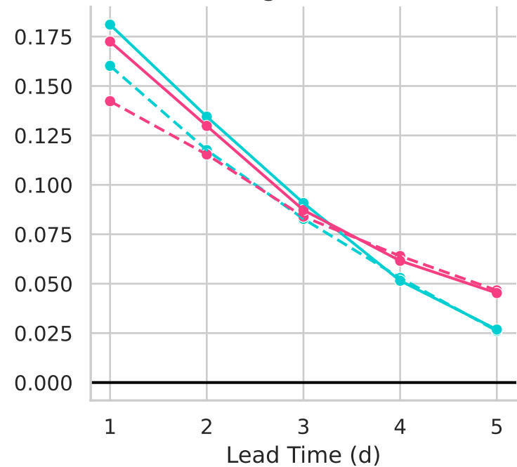
Variogram Score
