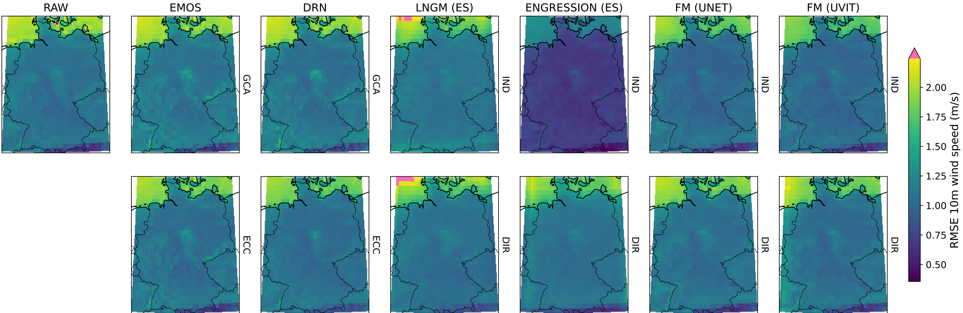
Mean Spatial RMSE - 10m wind speed
