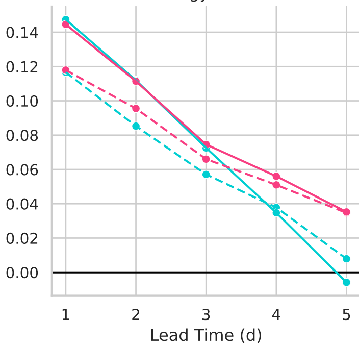
Energy Score
