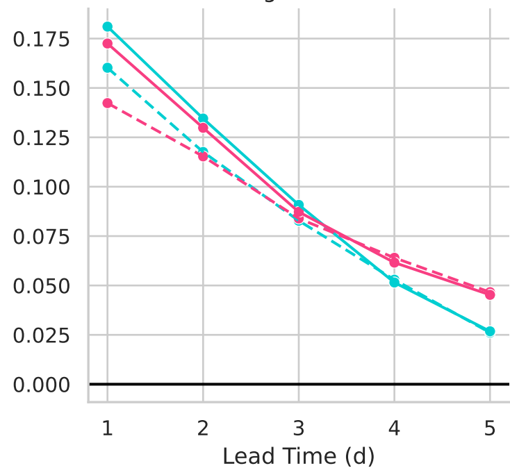
Variogram Score
