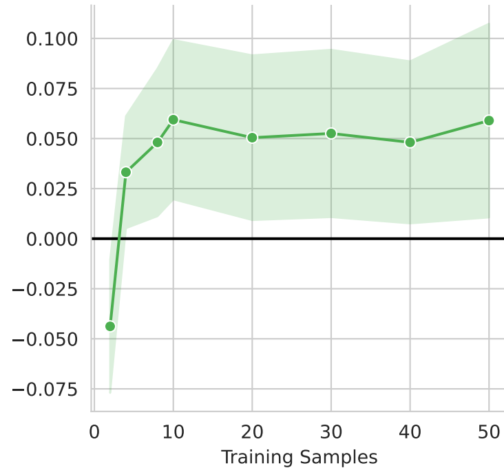
Variogram Score
