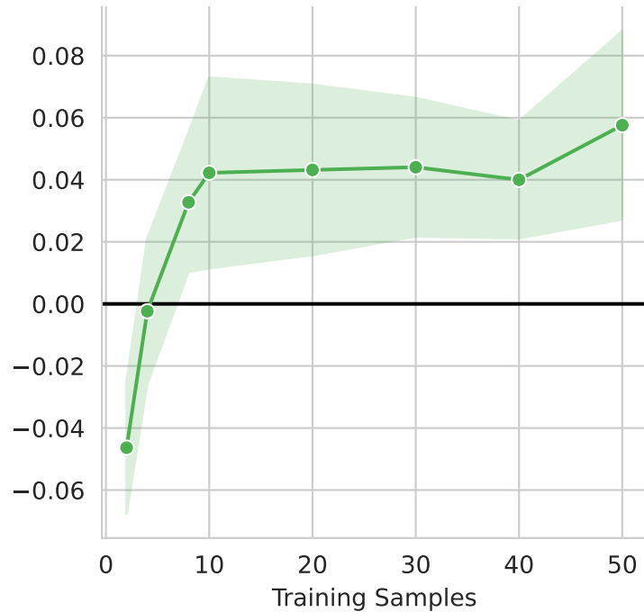
CRPS
