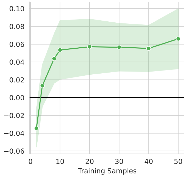
Energy Score
