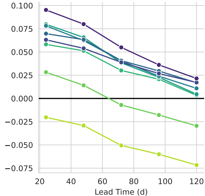
CRPS
