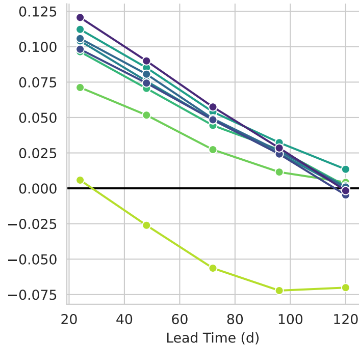
Variogram Score
