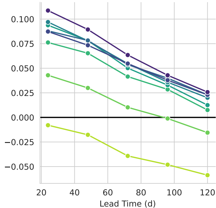
Energy Score
