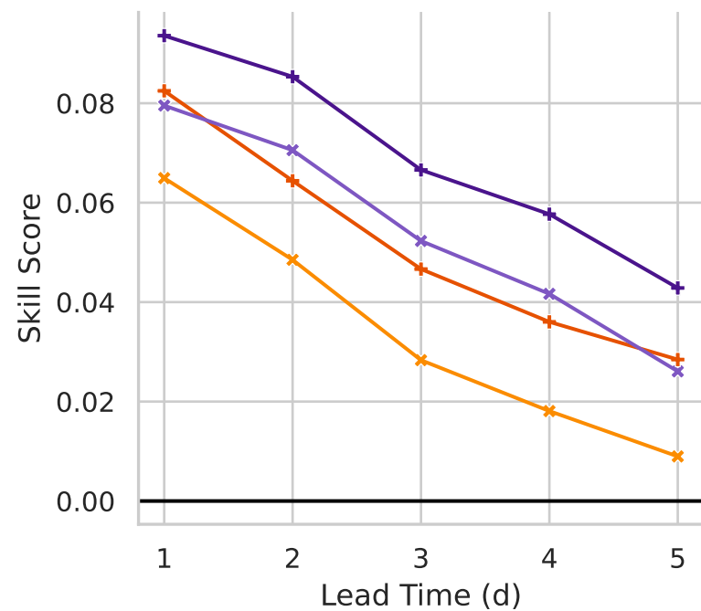
CRPS
