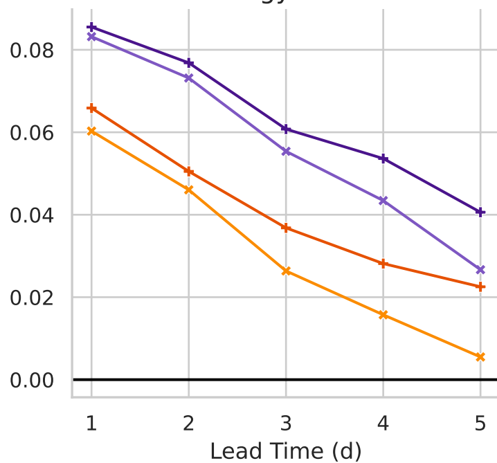
Energy Score
