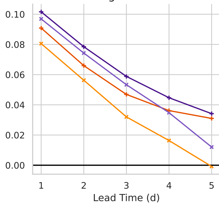
Variogram Score
