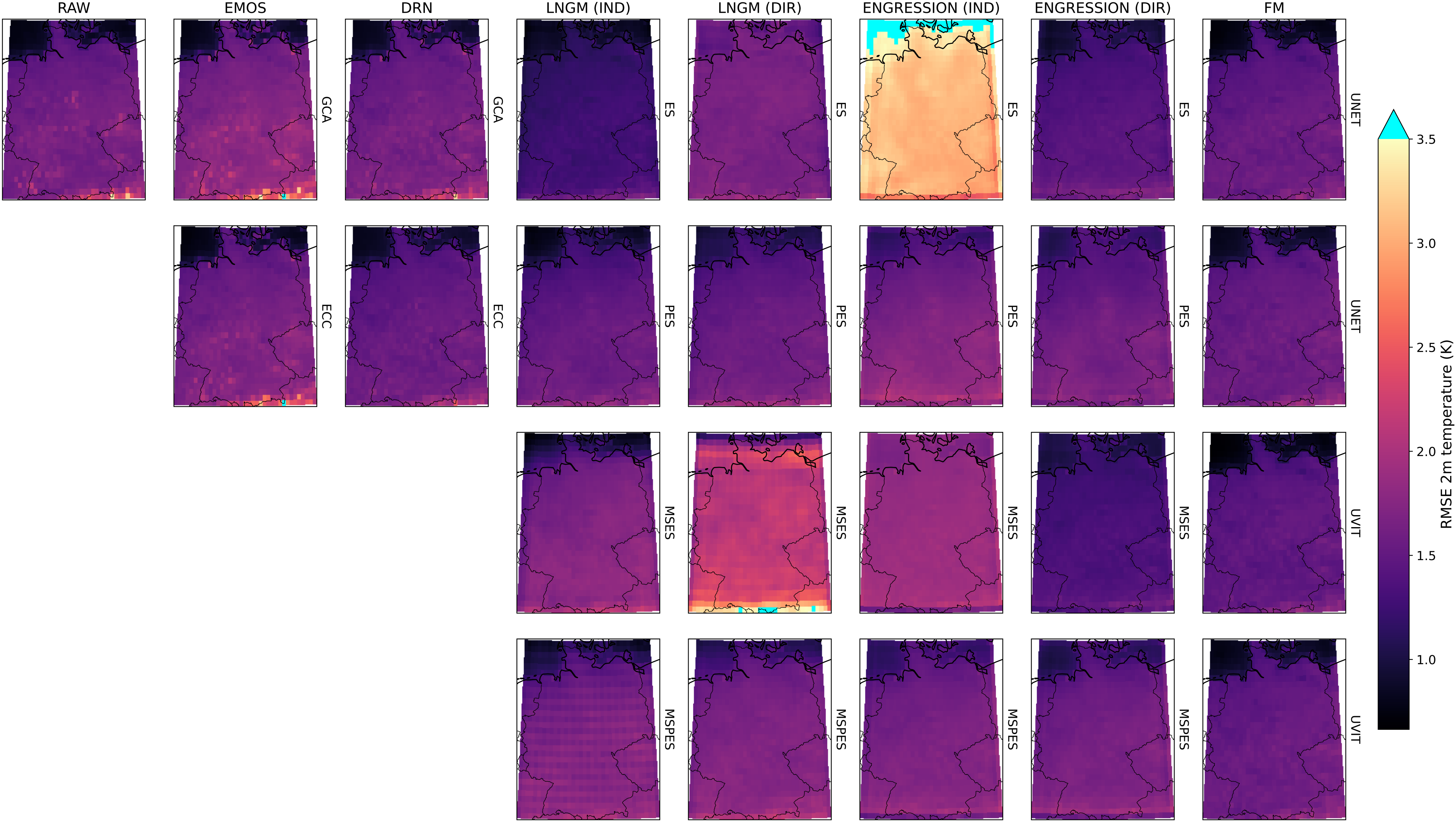
Mean SpatialRMSE - 2m temperature
