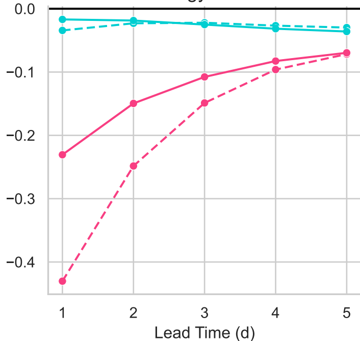
Energy Score
