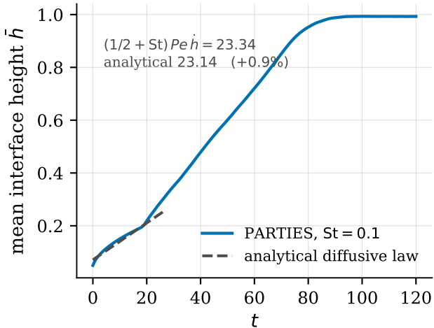
(a) interface height
