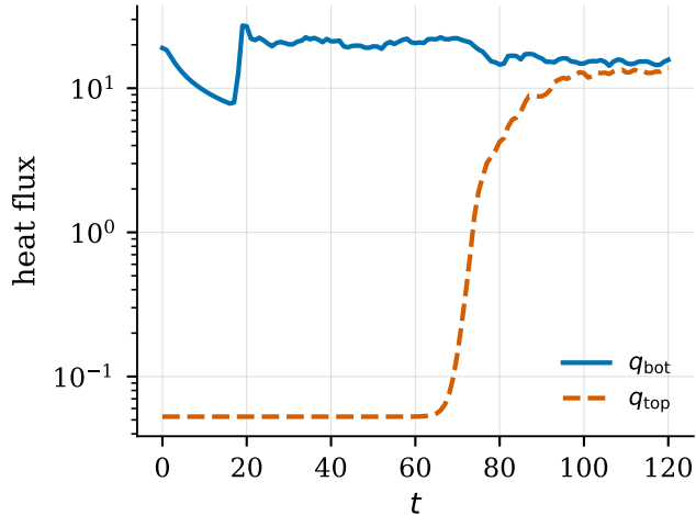
(b) boundary heat fluxes
