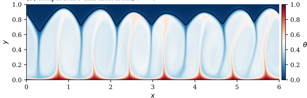
(b) temperature and melt front, t = 70
