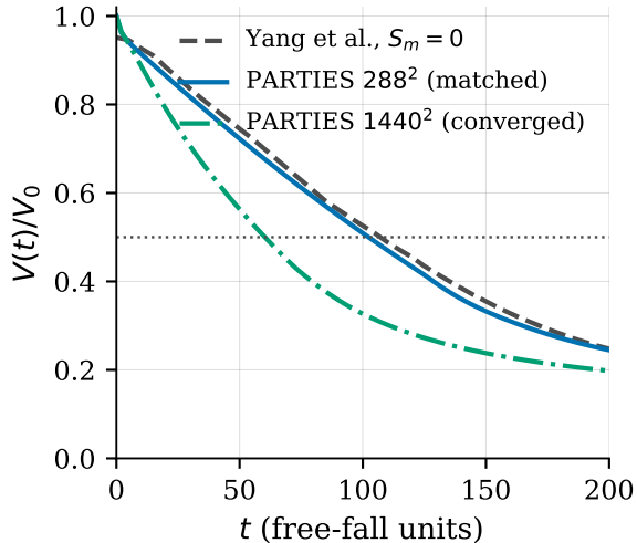
(b) ice volume, freshwater
