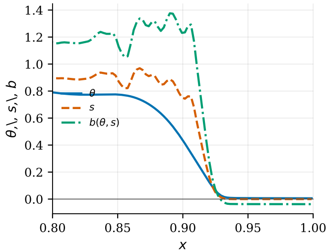
(b) mid-height profiles, t = 100
