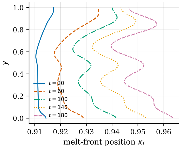
(a) melt-front evolution
