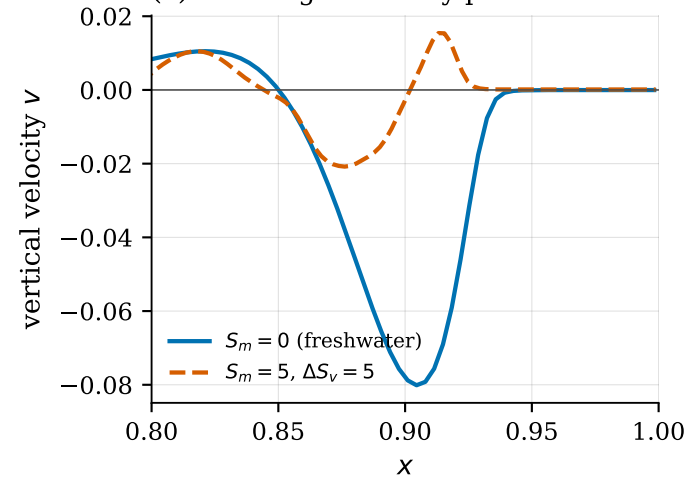
(a) mid-height velocity profile
