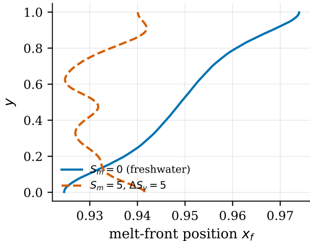
(b) melt-front shape
