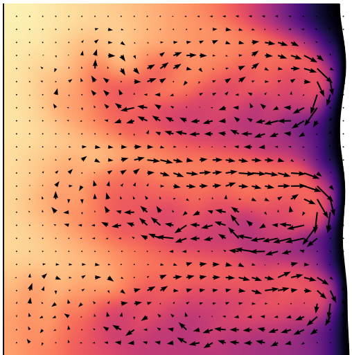
temperature \theta
