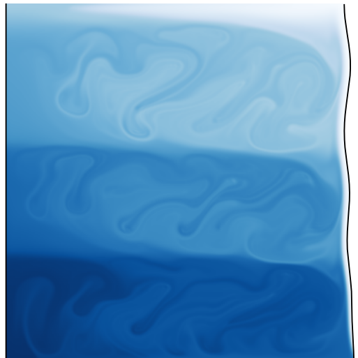
salinity s
