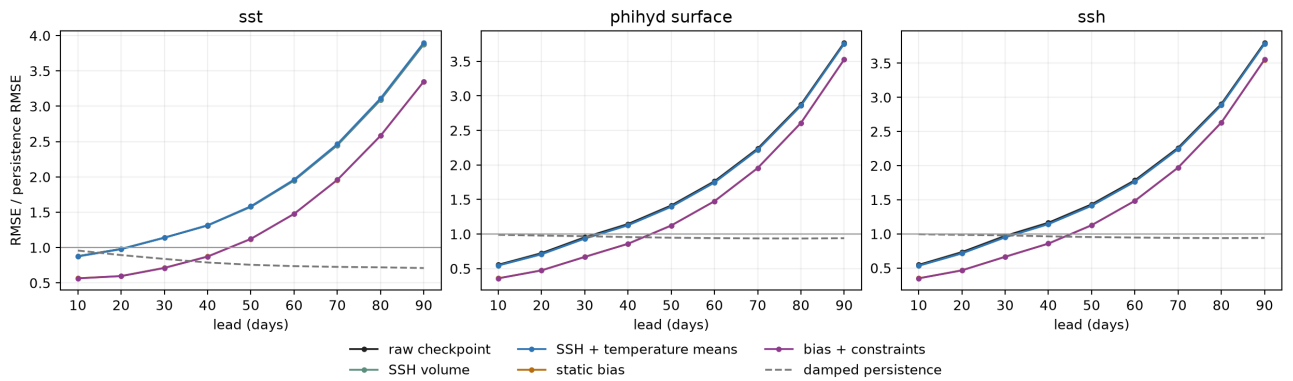
Frozen-checkpoint slow-field RMSE relative to persistence. Exact SSH/temperature mean constraints alone overlap or slightly worsen the raw curve; static-bias subtraction plus constraints delays the crossing and improves the AUC, but misses the predeclared 20% material-correction branch by 0.75 percentage points.
