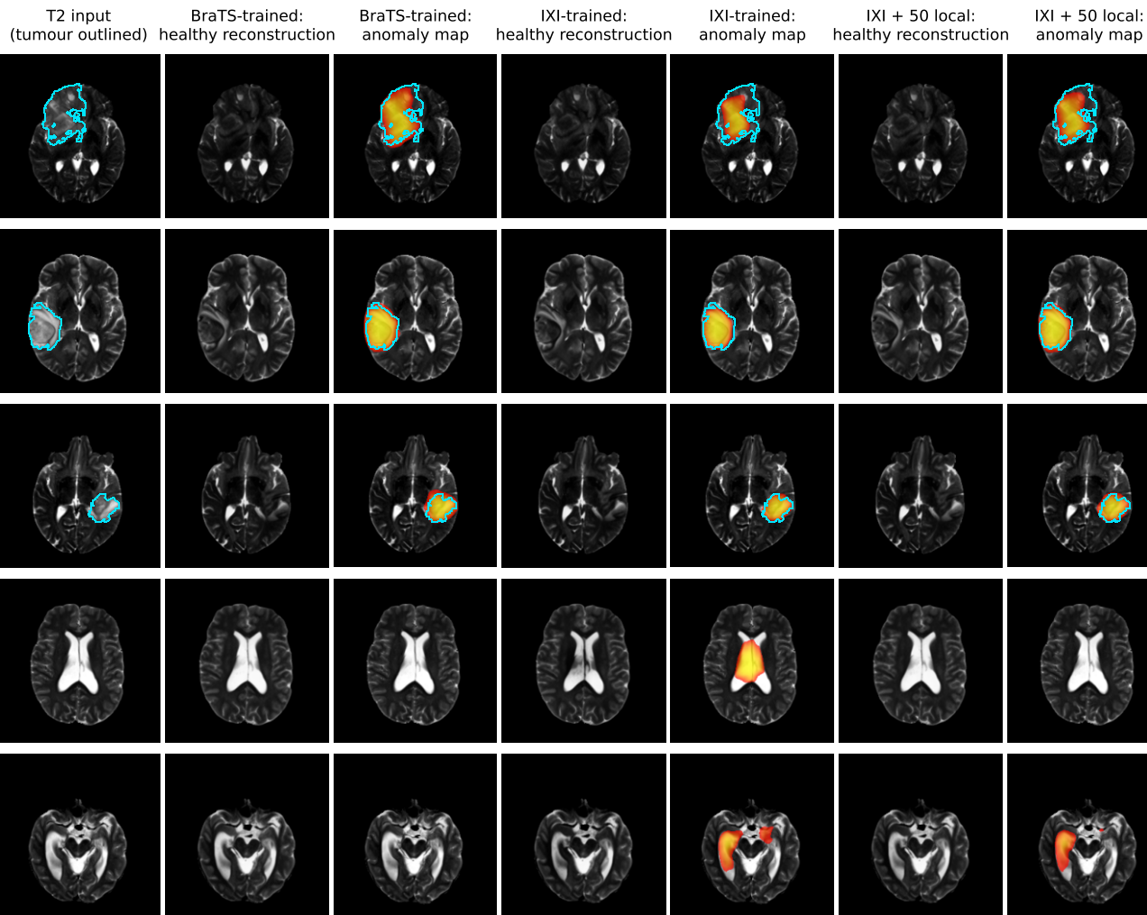
BraTS 2021 test slices. Anomaly maps thresholded where \leq 5\% of tumour-free validation slices fire.
