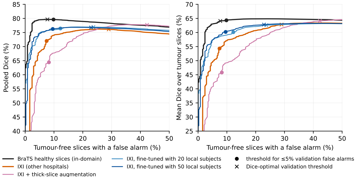
Dice against false alarms over all thresholds (BraTS 2021 test subjects, T2)
