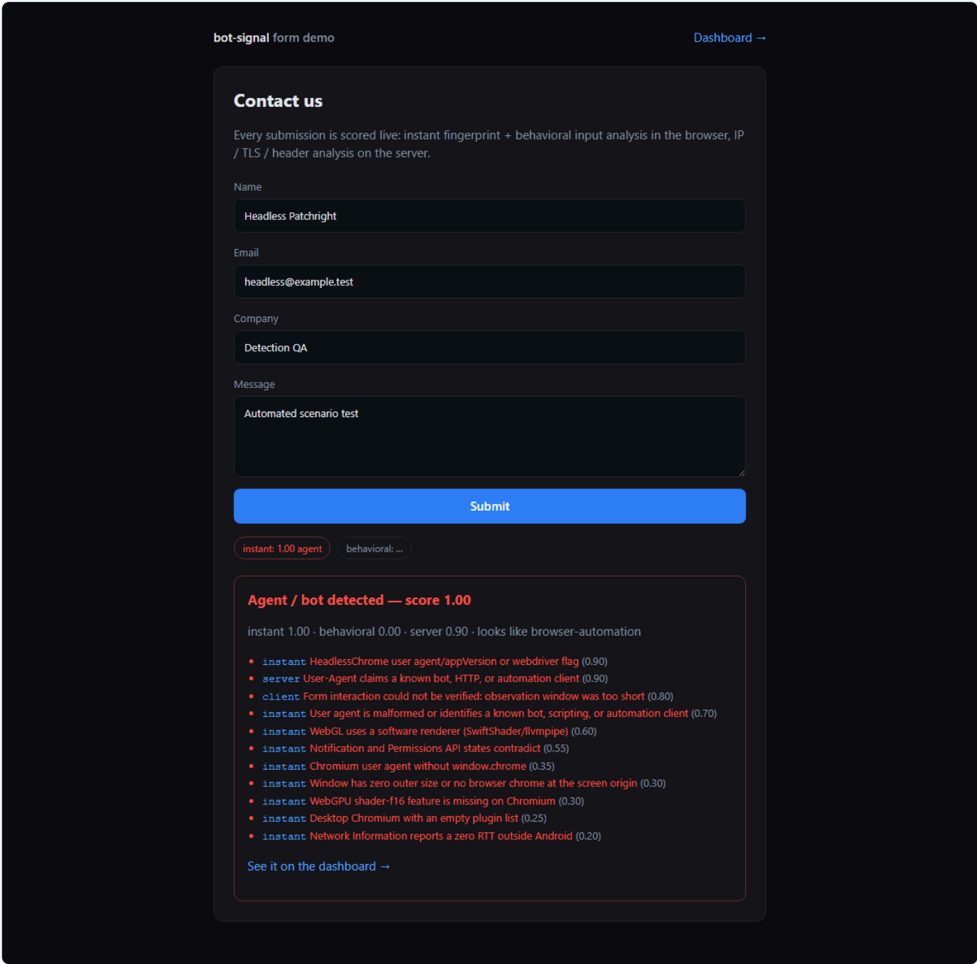
Standard headless automation: correctly classified AGENT, score 1.00.
