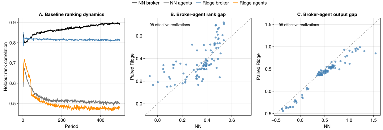
Figure R5: Direct paired-Ridge comparison. Panel A uses the 50 common baseline seeds. Panels B and C give one point to each of the 98 effective realizations. Dashed lines mark equal NN and Ridge values.
