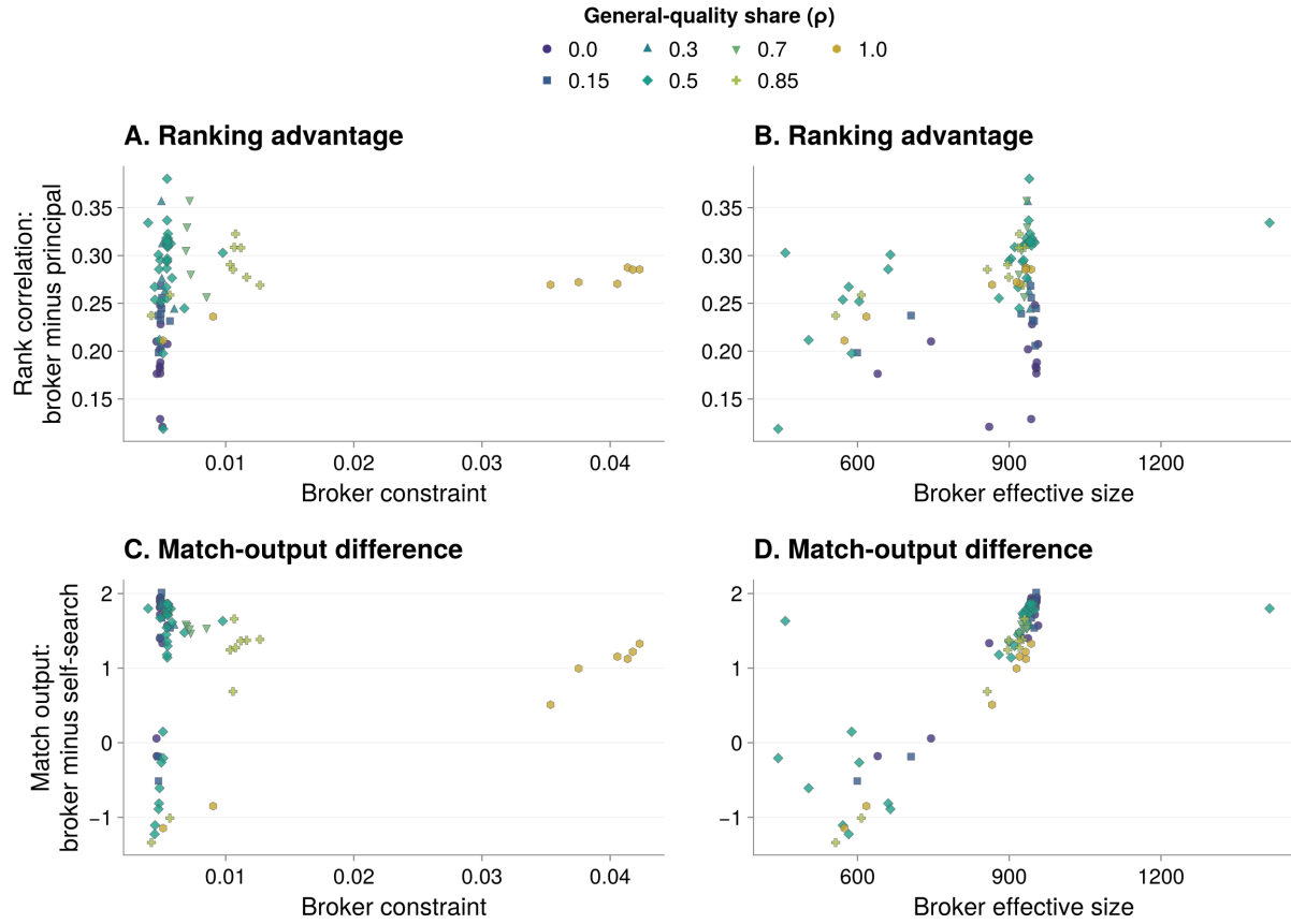
Figure S7: Ranking and output differences by alternative structural measures. Points show ensemble late means for 80 regimes. C–D compare mean realized output per completed match (brokered minus self-search), before costs and fees.
