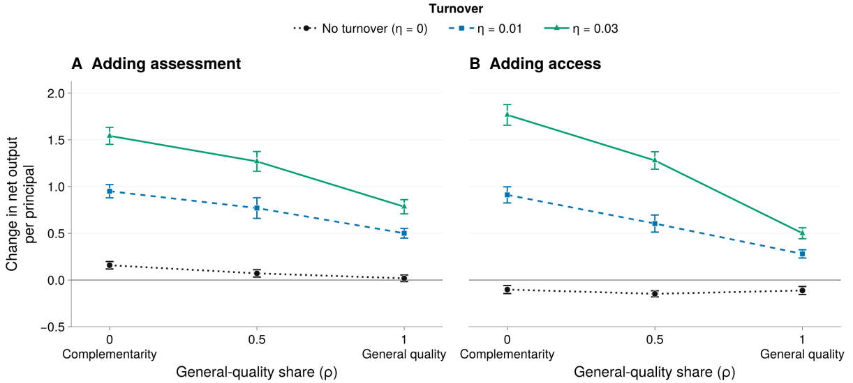
Figure S4: Contributions of assessment and access across matching composition. Late-mean differences paired by seed: A, full service minus access-only; B, full service minus assessment-only. Parameters other than matching composition and turnover remain at baseline. Points average 20 seeds per regime; bars show pointwise 95% Monte Carlo intervals. Connecting lines are visual guides.
