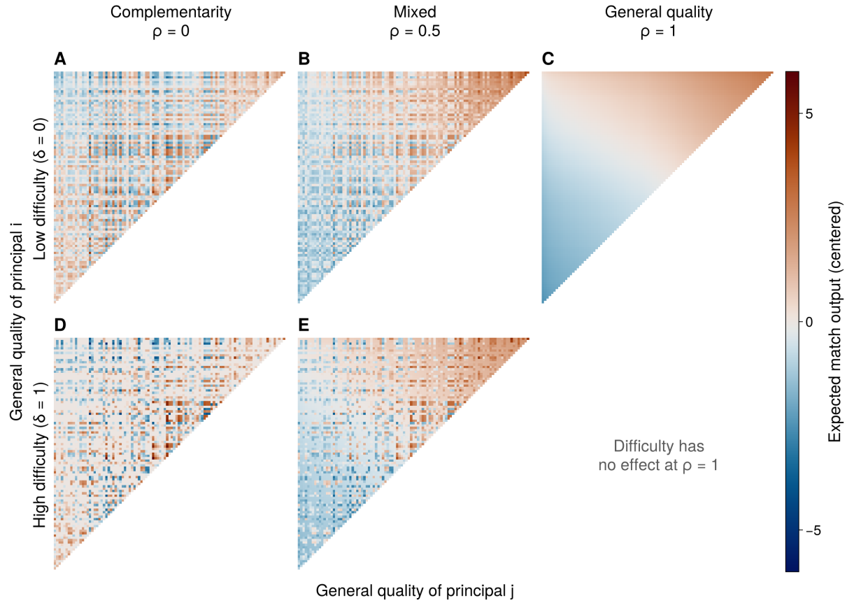
Figure S2: Expected match output across pairs of principal types. 100 types selected at evenly spaced general-quality ranks from realization 1 (1000 principals). Types and matching-function objects c , A , and B are fixed across panels. General quality increases rightward and upward. Upper triangles exclude self-matches; colors show expected output minus the grand mean, without match noise.
