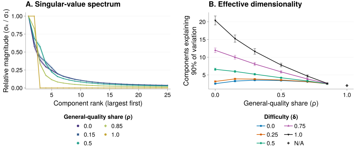
Figure S3: Dimensionality of expected match output. Centered expected-output matrices without match noise, summarized over 50 independent realizations. Types and matching-function draws are fixed within each realization as \rho and \delta vary. A: the first 25 singular values at \delta = 0.5 , divided by the largest within each realization. B: the fewest components accounting for 90% of the sum of squared singular values. Lines and markers are means; ribbons and whiskers show pointwise 95% Monte Carlo intervals. N/A denotes pure general quality ( \rho = 1 ), where difficulty is inapplicable.
