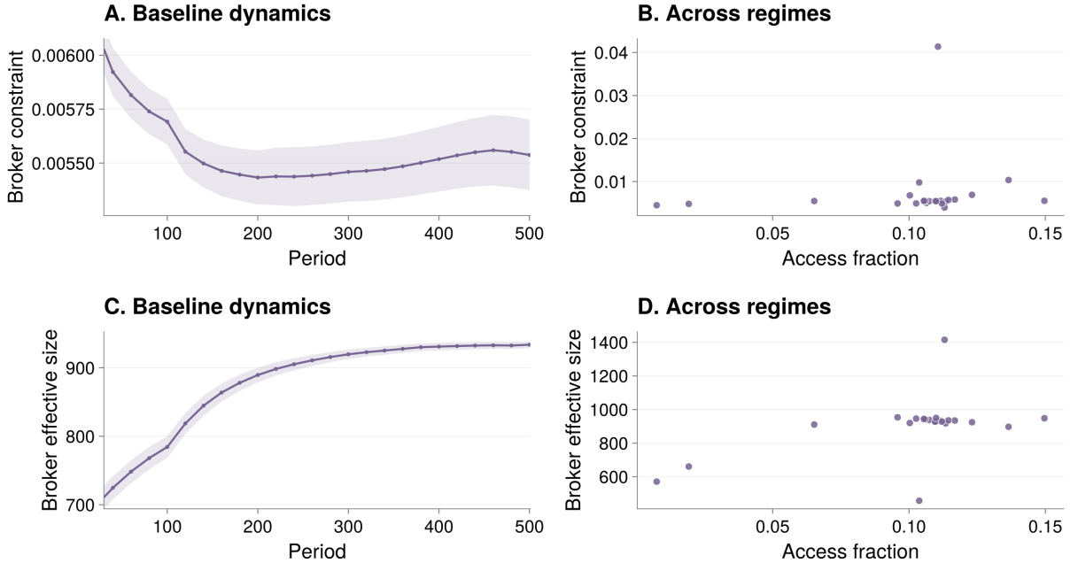
Figure S6: Alternative structural measures over time and against access. A and C: baseline measures recorded every 20 periods and smoothed within each seed using a 5-observation rolling mean, shown from t = 30 . Lines are ensemble means; ribbons show pointwise 95% Monte Carlo intervals. B and D: ensemble late means for the 26 regimes that vary one parameter at a time from baseline.
