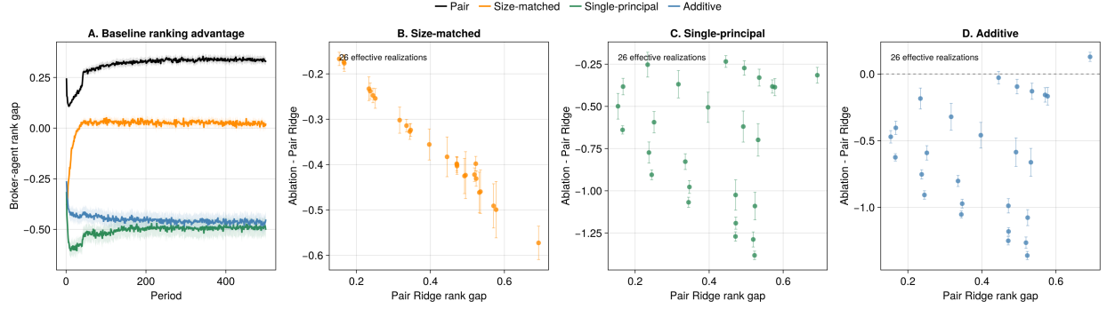
Figure RA1: Ridge broker restrictions. Panel A shows the baseline broker-minus-principal difference in holdout rank correlation over time under base Ridge and the three restrictions. Lines are ensemble means over 50 common seeds; ribbons are pointwise 95% Monte Carlo intervals. Panels B–D show each restriction’s paired change from base Ridge across the 26 effective regimes, against that regime’s base Ridge mean. Whiskers are paired 95% Monte Carlo intervals for the mean seed-level change, and dashed lines mark no change.
