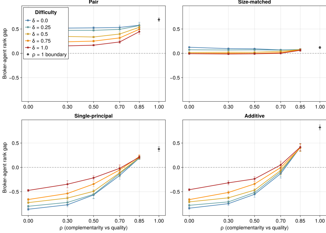
Figure RA2: Broker-agent rank-correlation gaps across the \rho \times \delta design. Each panel shows one Ridge broker variant, each line shows one value of \delta over \rho = 0 through 0.85, and markers are late-window seed means. The pure-quality boundary \rho = 1 , where \delta is inactive, is shown once and unconnected. The vertical scale is shared across panels, whiskers are 95% Monte Carlo intervals, and the dashed line marks a zero broker-agent gap.
