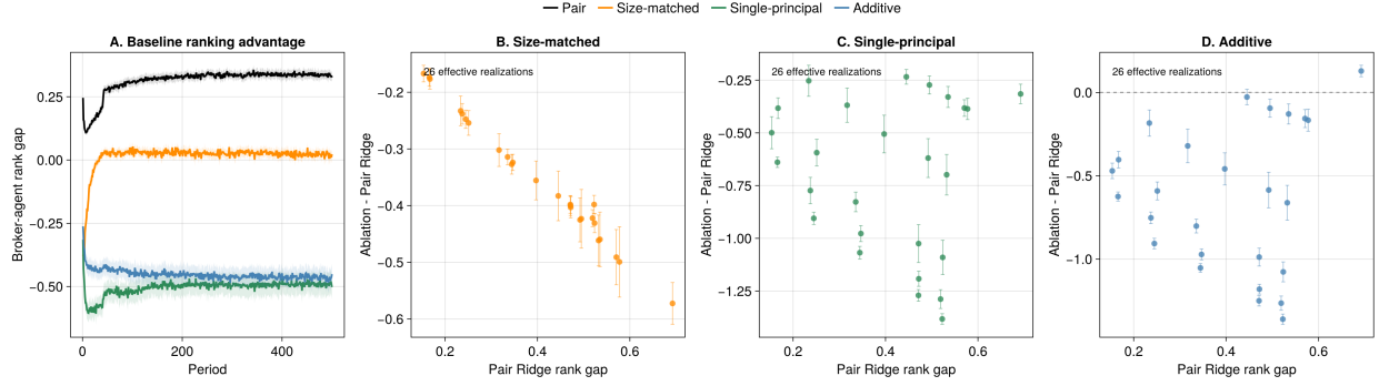
Figure RA1: Ridge broker ablations. Panel A uses all 50 baseline seeds. Panels B–D plot the paired ablation-minus-reference difference for each effective realization against its paired-Ridge mean. Ribbons in Panel A are pointwise 95% Monte Carlo intervals. Whiskers in Panels B–D are 95% intervals for the mean seed-level difference, and dashed lines mark no difference.
