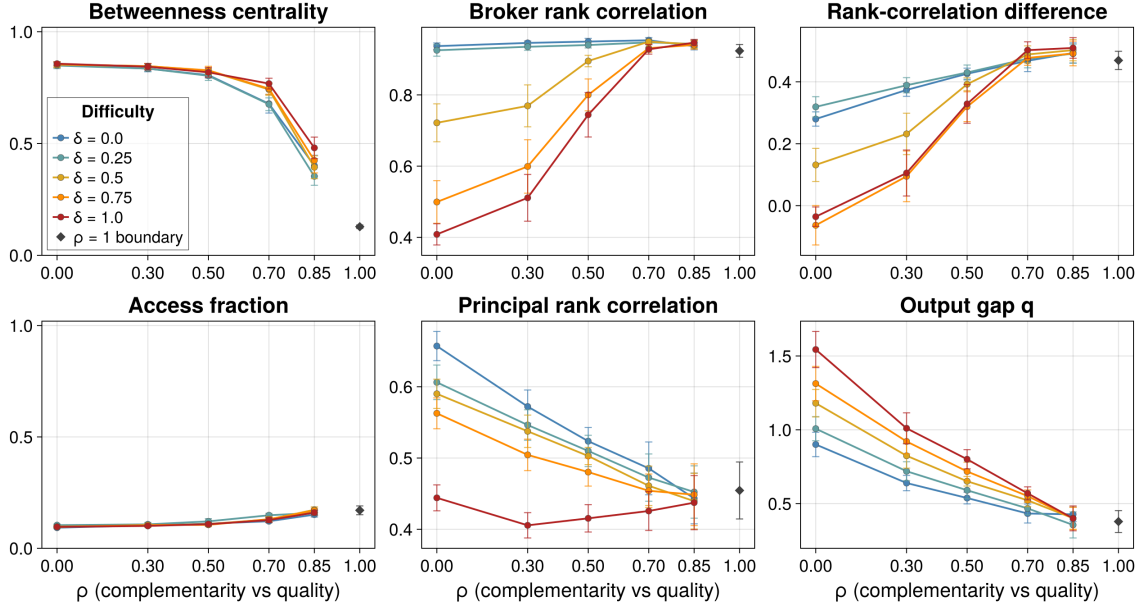
Figure 3: Outcomes across the matching problem (\rho \times \delta) . Six outcomes across the \rho \times \delta grid; one line per difficulty level \delta , each spanning \rho = 0 through 0.85. The pure-quality boundary \rho = 1 , where \delta has no effect, is one separate regime shown once and unconnected. The figure therefore displays all 26 regimes in the design. Each marker is a late-window mean over that regime’s seeds; whiskers are 95% Monte Carlo intervals. The reported difference in holdout rank correlation is broker minus principal; the output gap is broker channel minus self-search.
