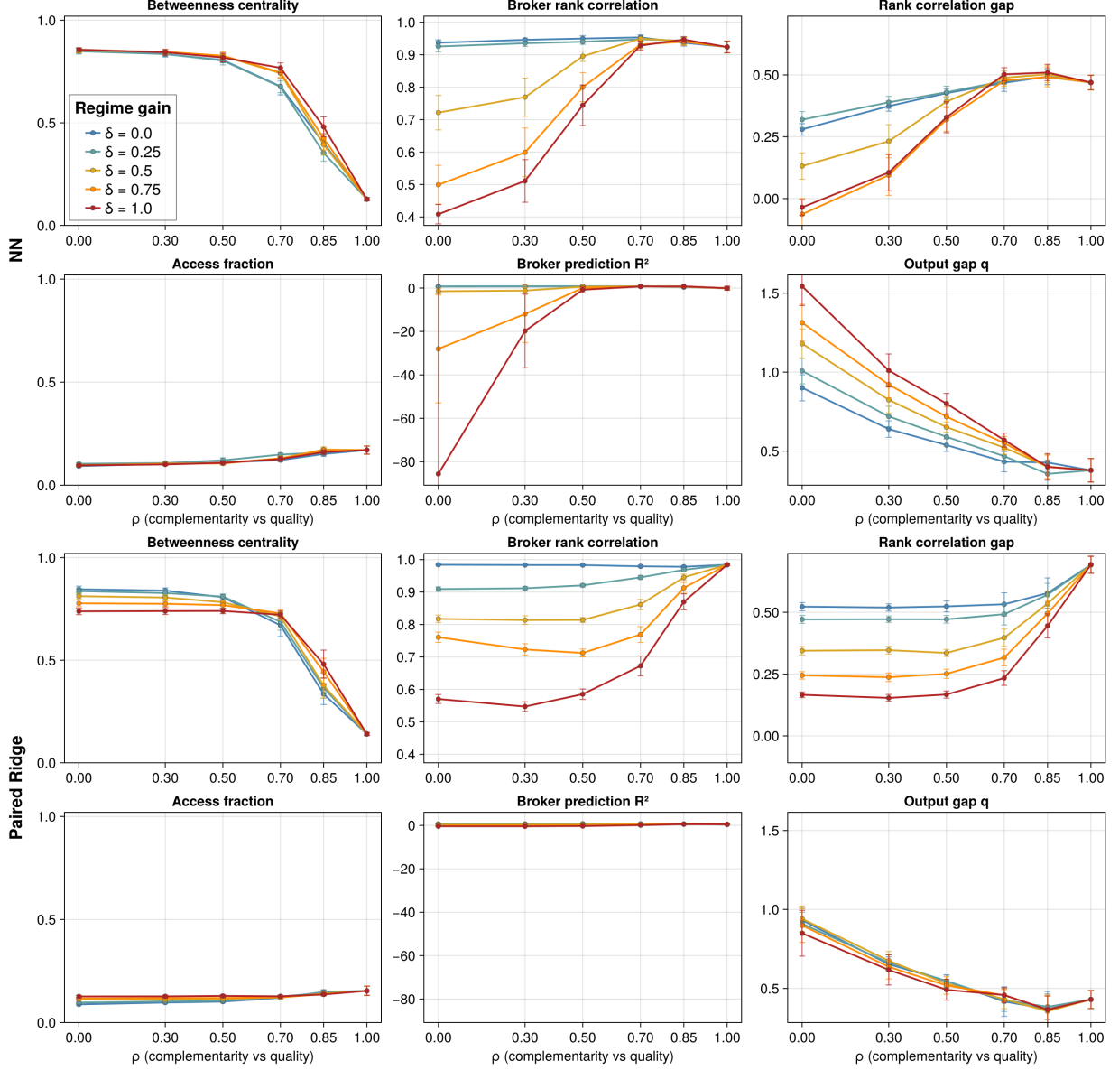
Figure R2: Outcomes across the \rho \times \delta matching grid under NN (top two rows) and paired Ridge (bottom two rows). Each line is a value of \delta ; each marker is a grid coordinate's late-window seed mean. Corresponding NN and Ridge panels use the same vertical scale. Whiskers are 95% Monte Carlo intervals. Coordinates that map to the same effective realization share the same estimate and receive no additional analytical weight.
