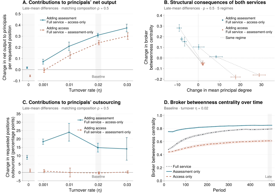
Figure 2: Brokerage with access, assessment, or both. All panels use \rho = 0.5 and \delta = 0.5 , with other parameters at baseline except turnover. A–C show late-mean contributions of adding assessment (full service minus access-only, blue circles) and adding access (full service minus assessment-only, orange triangles) across 5 turnover rates. A: change in net output to principals per requested position. B: change in broker betweenness centrality against change in mean principal degree. Dashed grey lines connect the two contrasts within each regime. Degree includes each principal's tie to the broker when present. C: change in outsourcing, in percentage points. In A and C, zero turnover is shown separately, positive rates use a linear scale, and baseline turnover is shaded. Horizontal offsets separate series; connecting lines are visual guides. D: broker betweenness centrality at baseline turnover ( \eta = 0.02 ). Lines join unsmoothed ensemble means measured at t = 20, 40, \dots, 500 ; shading marks the late window. Bars and ribbons show pointwise 95% Monte Carlo intervals, paired by seed in A–C. Each service version uses 50 seeds at baseline and 20 elsewhere.
